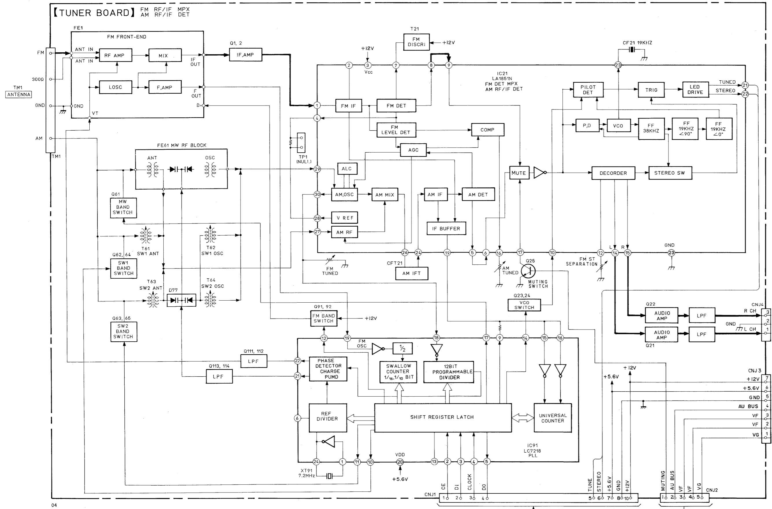
4-1. BLOCK DIAGRAM
